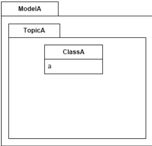
INTERLIS model
