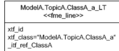
FME feature schema
