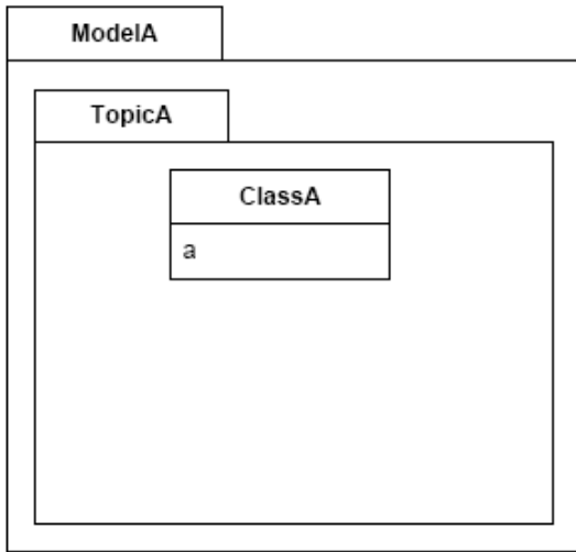
INTERLIS model
