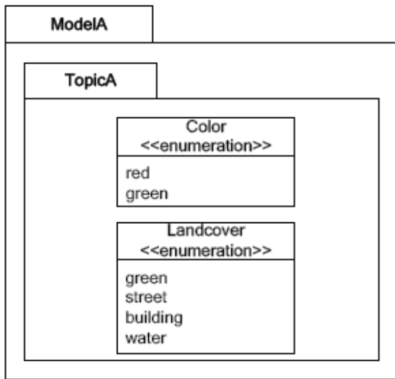
INTERLIS model
