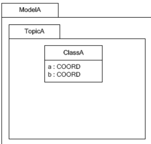
INTERLIS model
