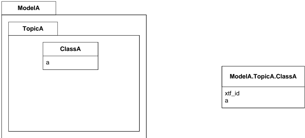
FME feature schema
