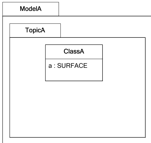
INTERLIS model
